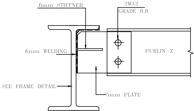
PURLIN JOINT WITH COLUMN N.T.S
