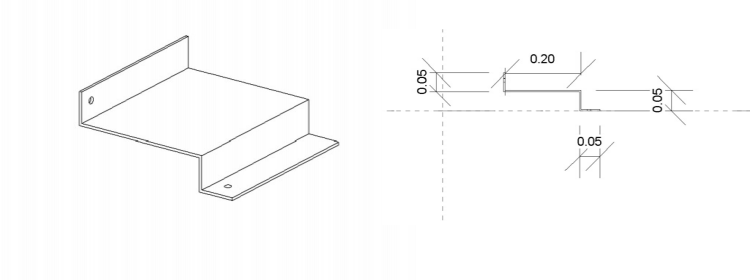
DRAIN LINE COVER DETAIL
