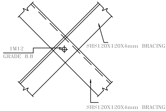
BRACING INTERSECTION DETAILS N.T.S
