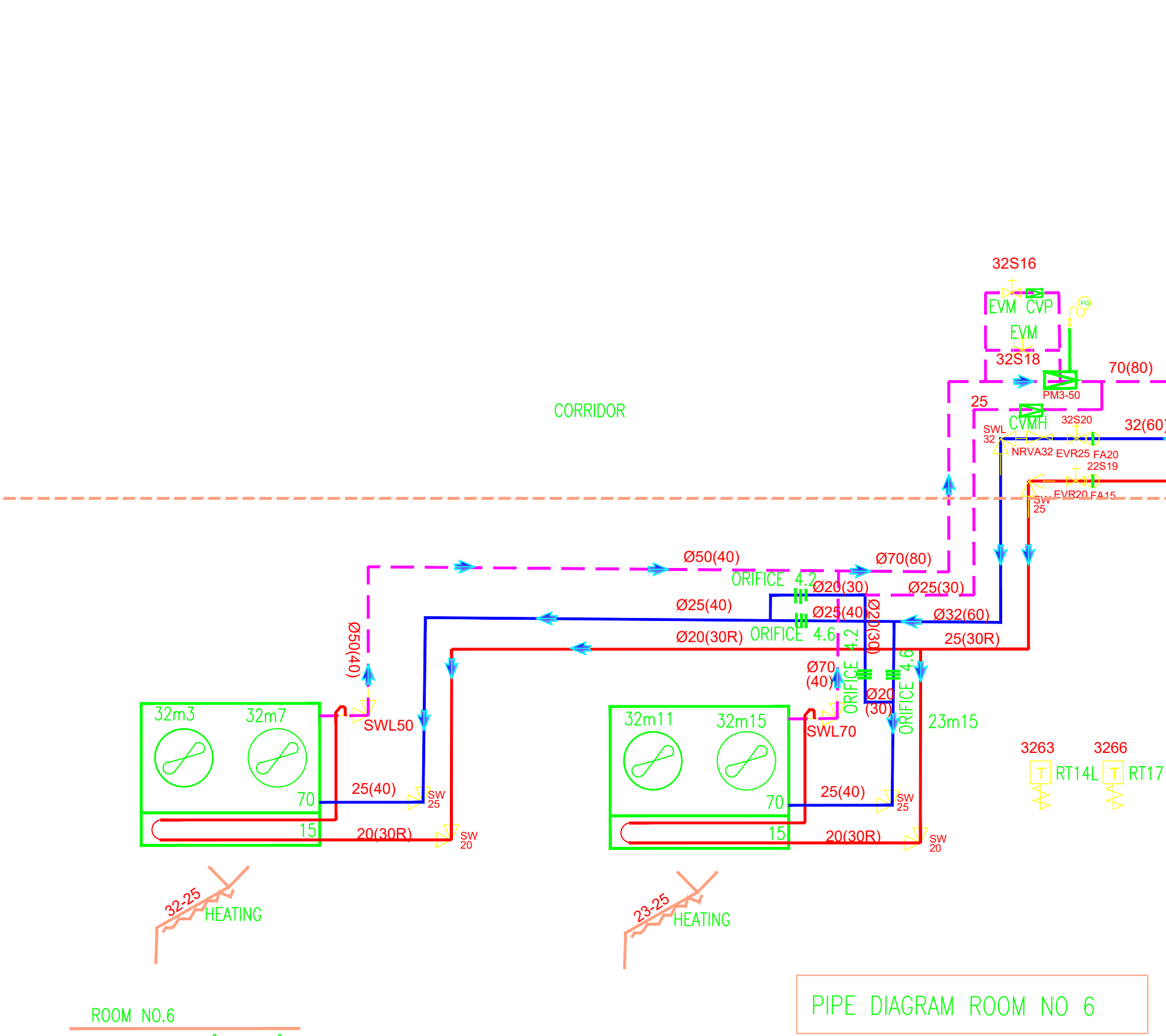
PIPE DIAGRAM ROOM NO 6
