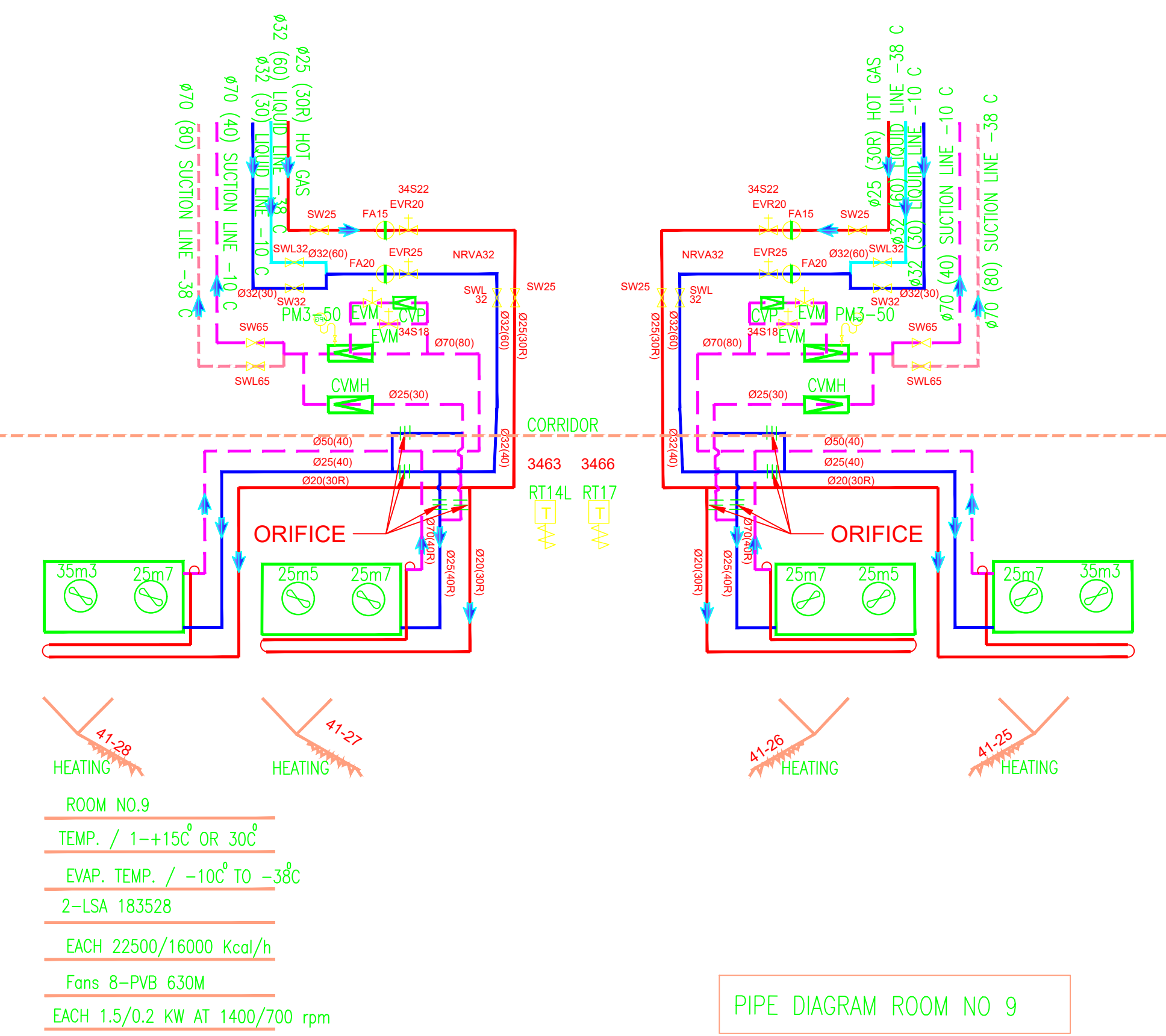
PIPE DIAGRAM ROOM NO 9
