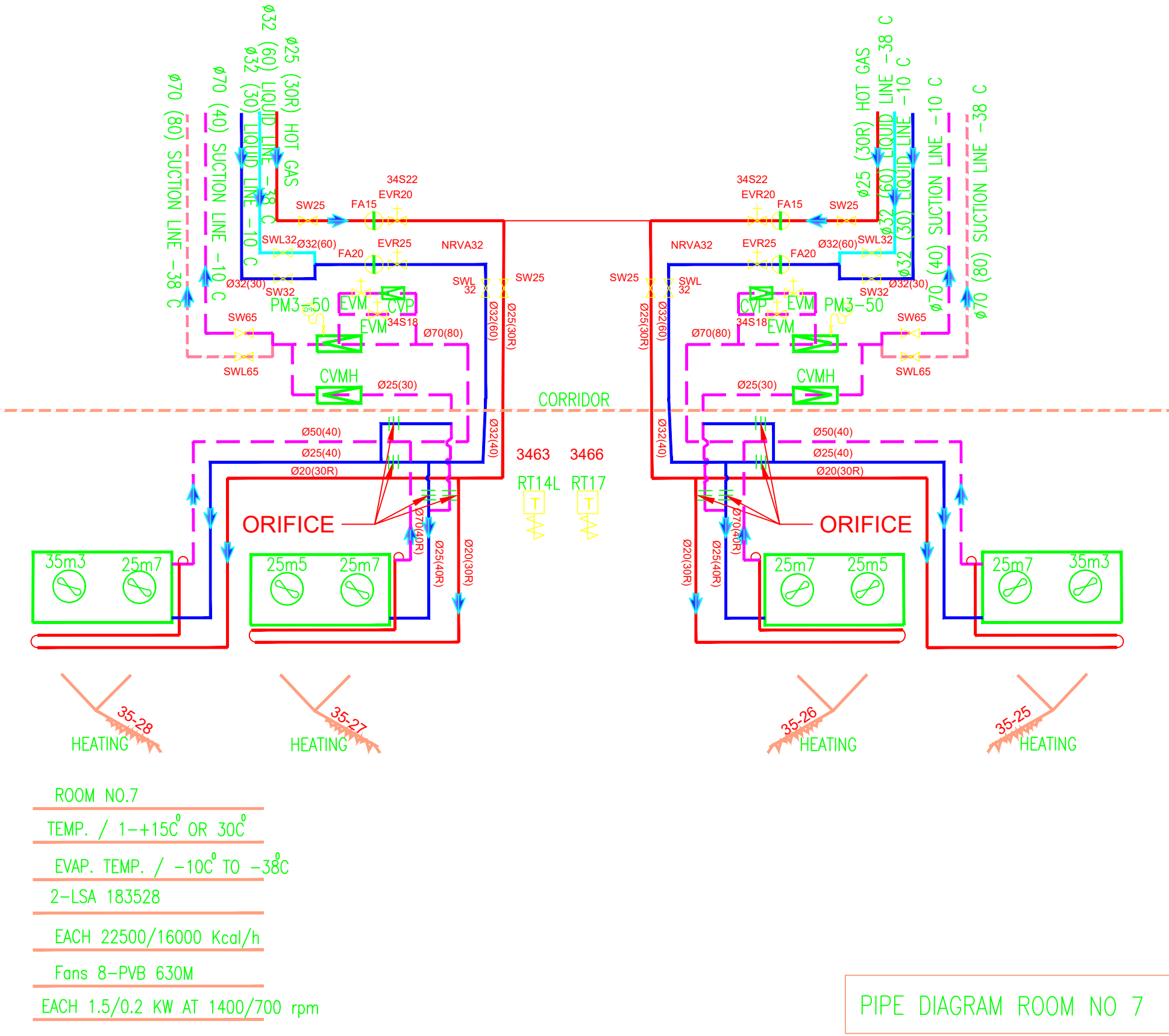
PIPE DIAGRAM ROOM NO 7
