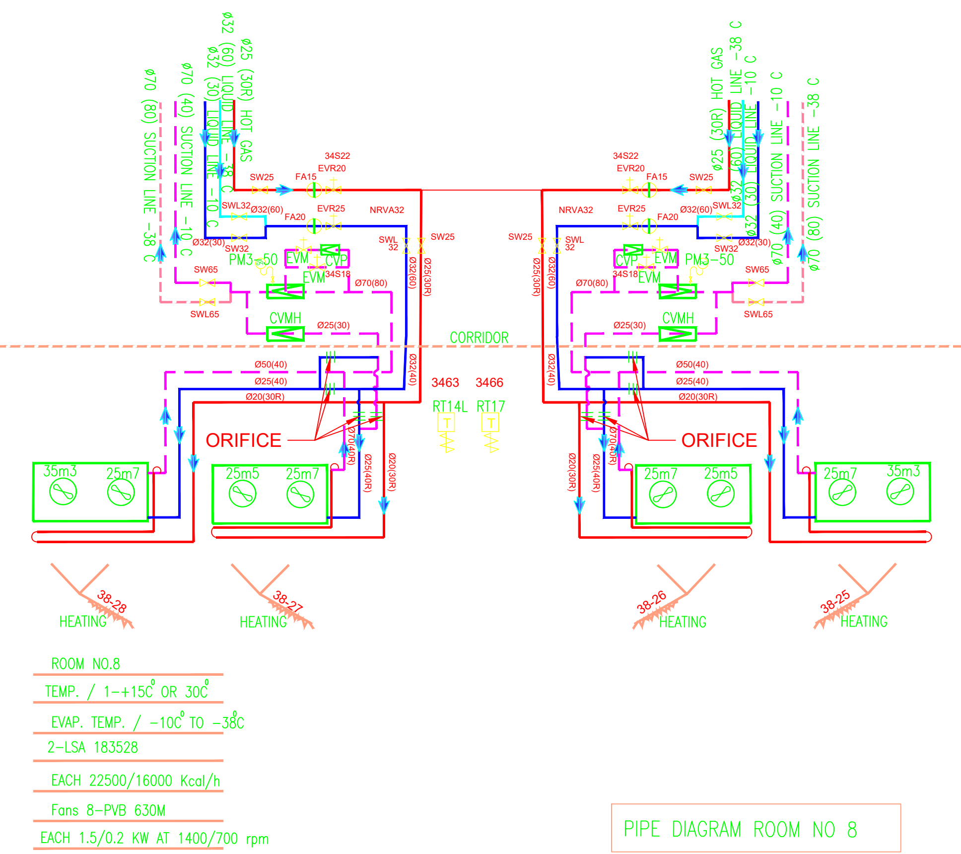
PIPE DIAGRAM ROOM NO 8
